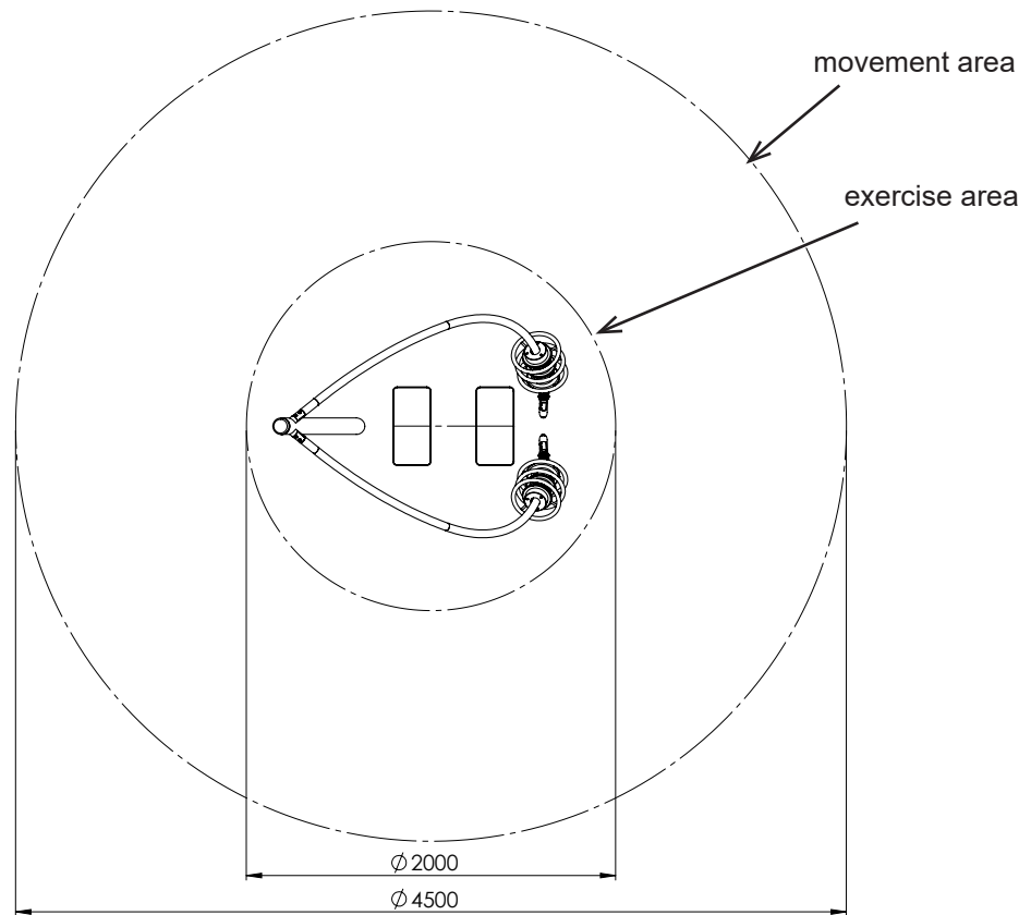
Diagram 3: Top view
